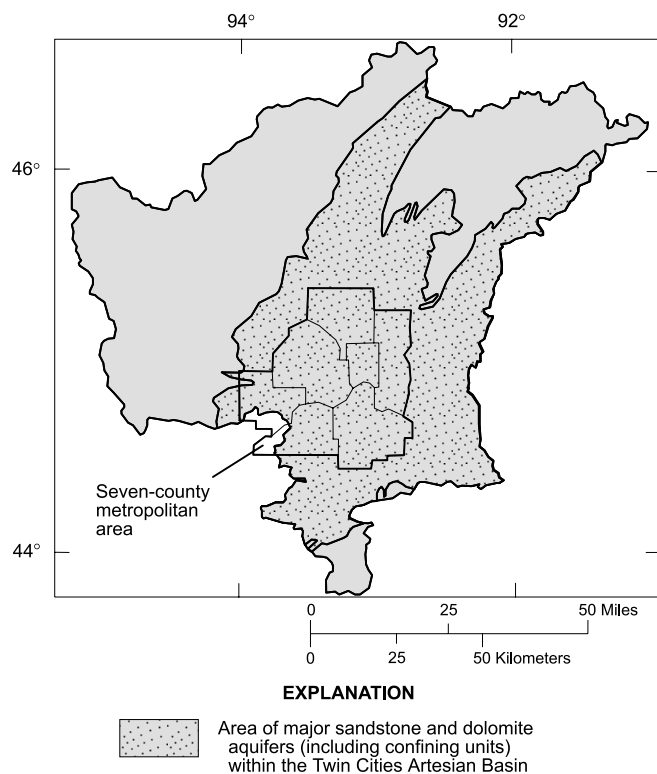
Figure 2. Major bedrock hydrogeologic systems in the Upper Mississippi River Basin study area in Minnesota and Wisconsin.
