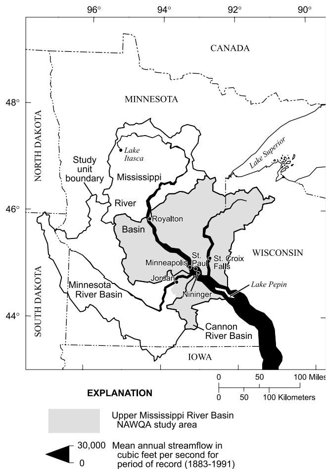
Figure 1. Upper Mississippi River Basin and NAWQA study unit.
