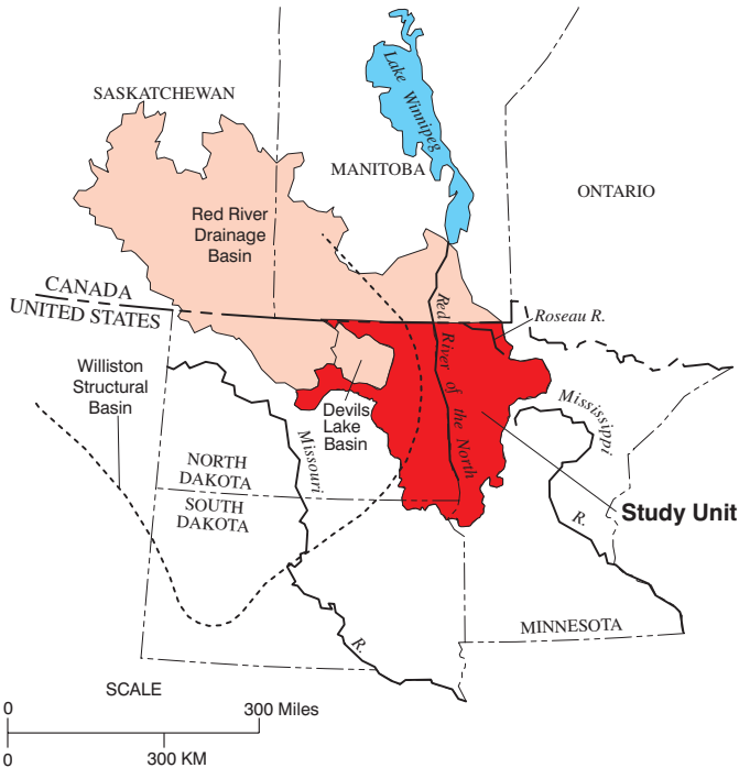
Figure 1.--Location of the Red River of the North Basin study unit.
