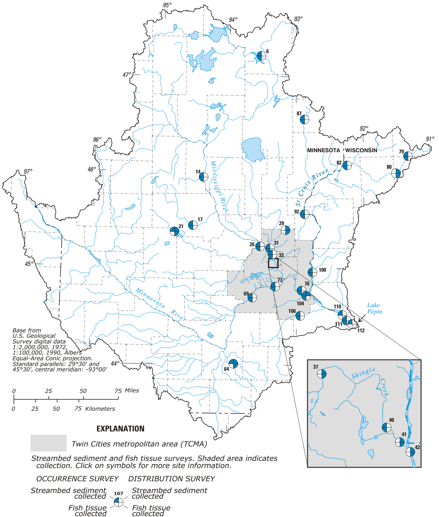
Figure 9.--Location of streambed sediment and biological tissue sampling sites in the Upper Mississippi River Basin study unit.
